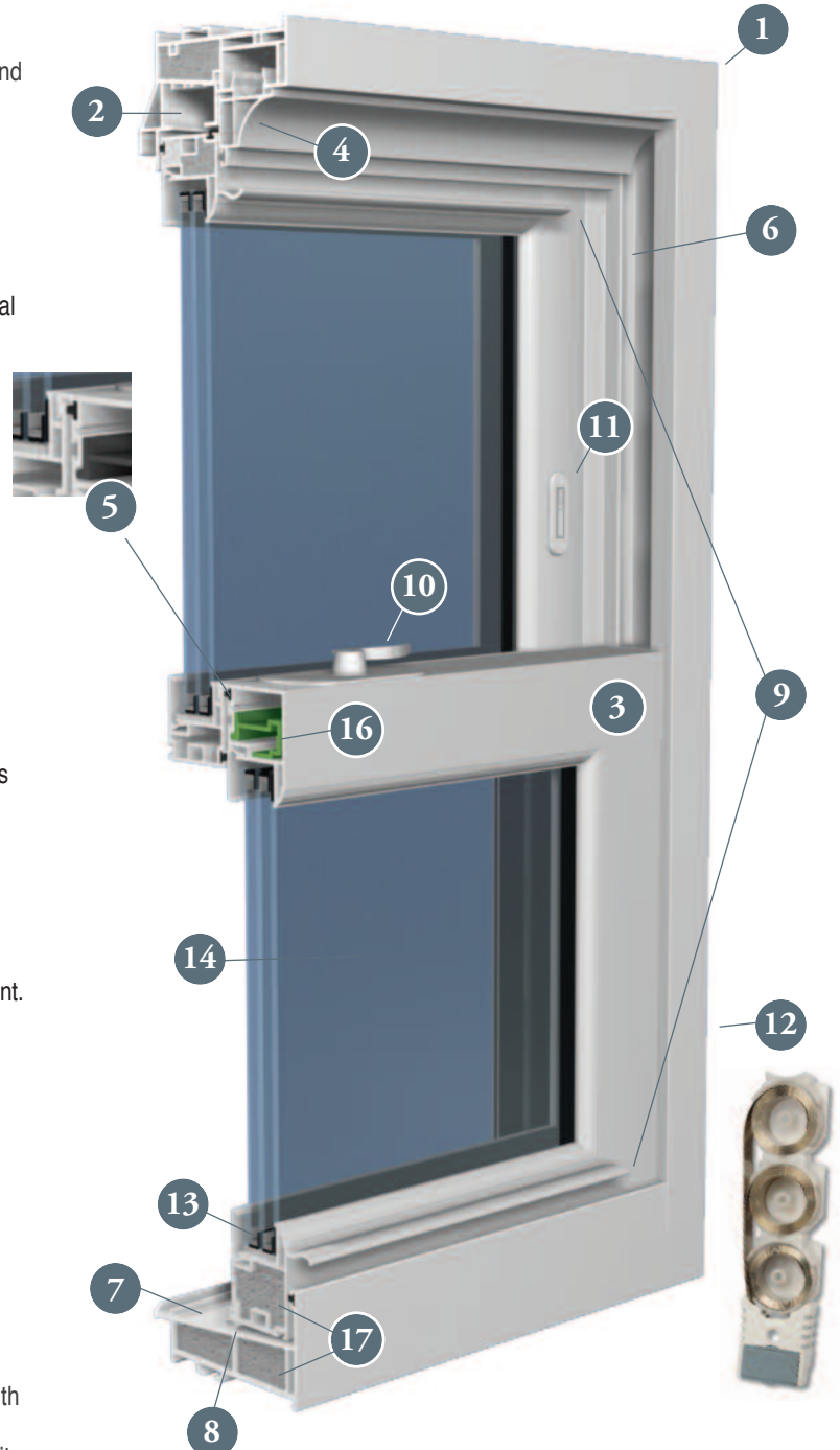
Hyde Park double hung shown in white with optional IntelliGlass Plus triple pane glass, optional ArmorCor fortification and optional IntelliFoam insulation.
